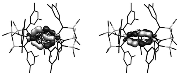
Figure 2. \alpha -Spin Kohn–Sham orbital representations of the two \delta -bonds in 2 : a) HOMO–2 (411a, –3.670 eV); b) HOMO–3 (410a, –3.766 eV).
